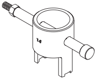
T-6 Motor Lock Ring Wrench/Spindle Puller
